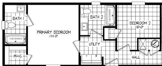
2-BDRM/2-BATH OPT
